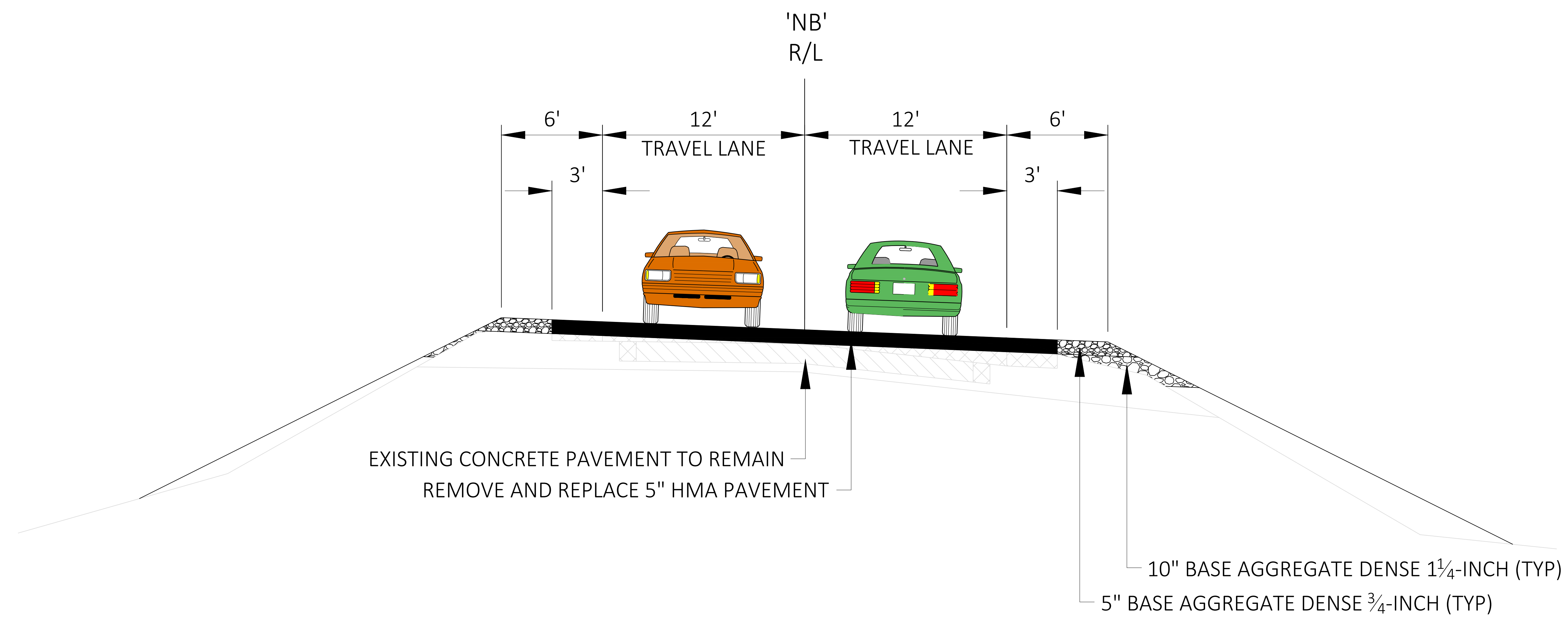
PROPOSED TYPICAL SECTION WIS 23 LUCY STREET TO MINERVA STREET
