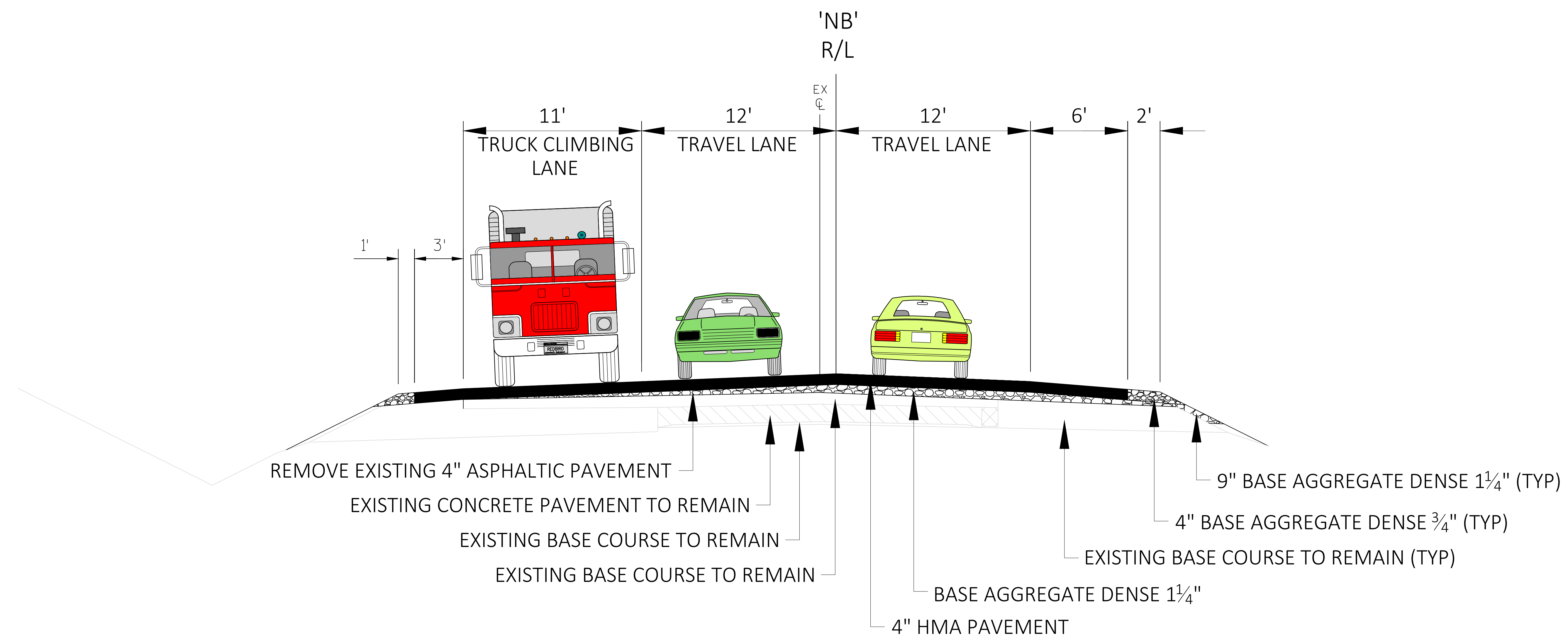
PROPOSED TYPICAL SECTION WIS 23 COUNTY SHOP ROAD TO CENTER HILL ROAD
