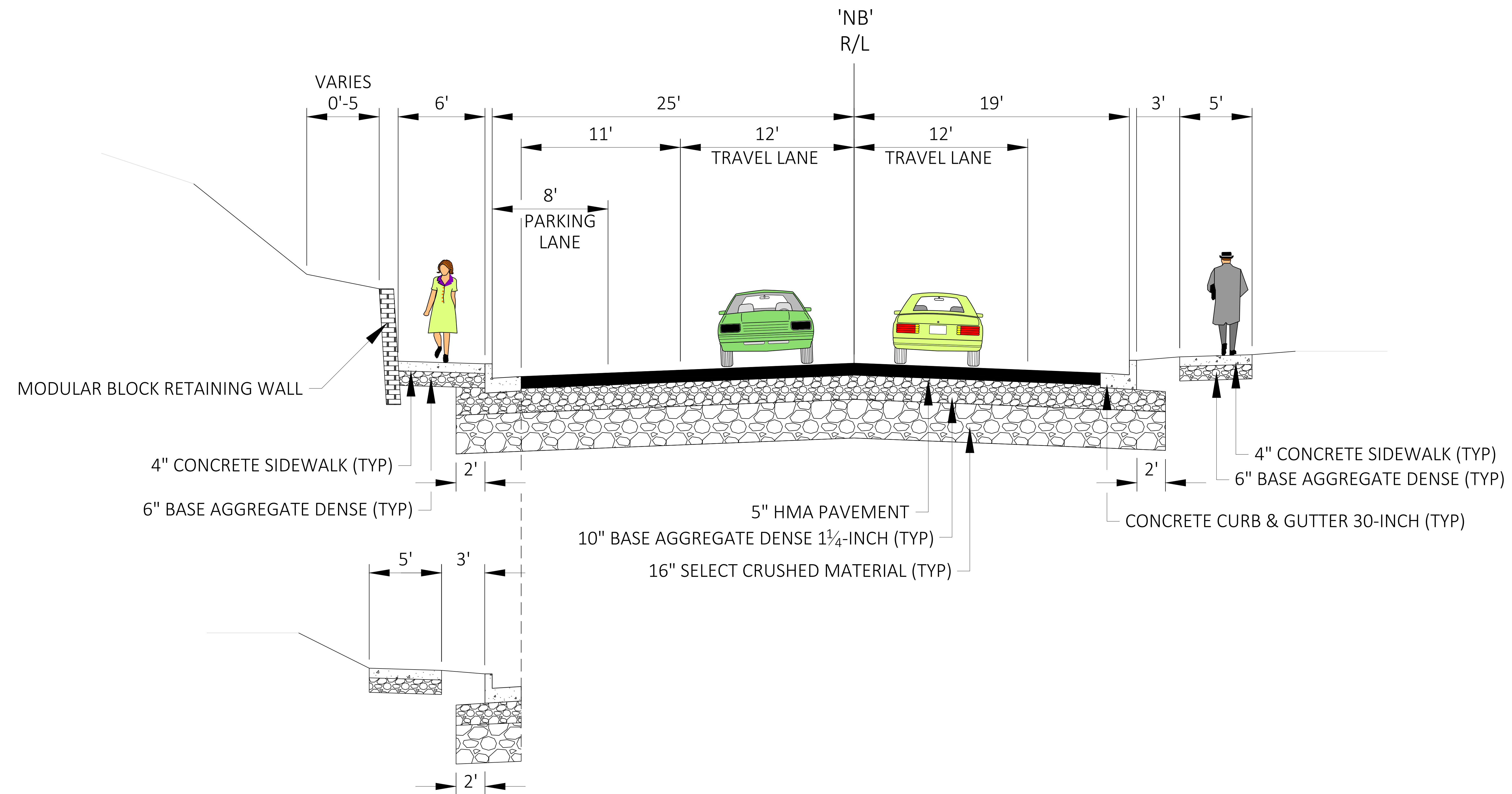
PROPOSED TYPICAL SECTION WIS 23 CENTER HILL ROAD TO PECATONICA RIVER BRIDGE
