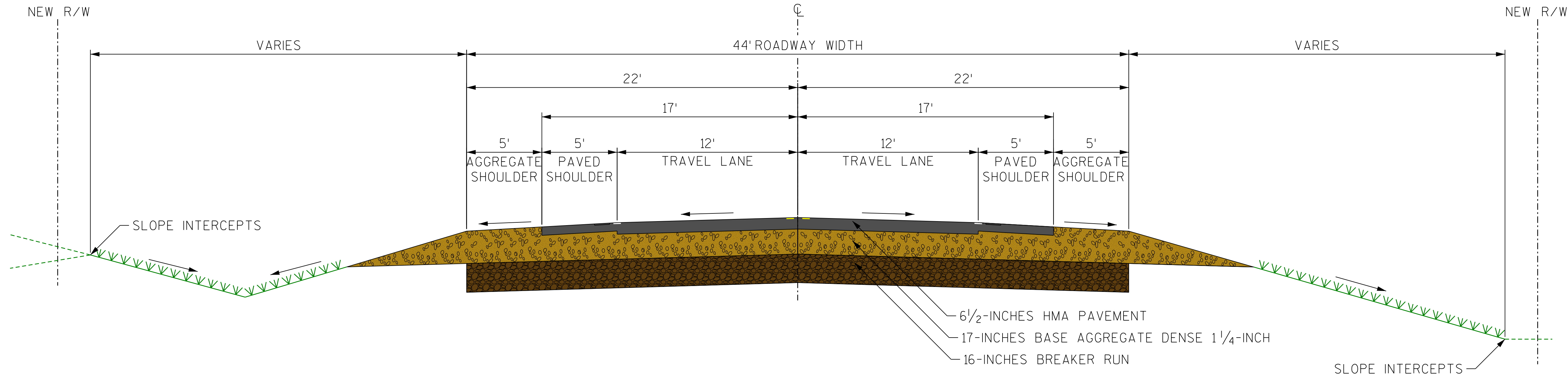
PROPOSED TYPICAL SECTION - WIS 76 BEGIN PROJECT - 0.6 MILES NORTH OF CTH G CTH JJ - END PROJECT
