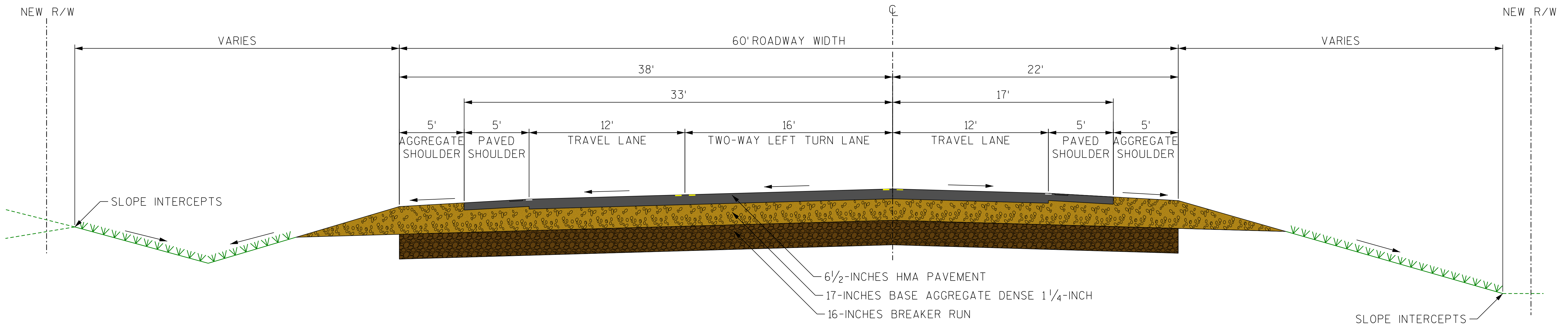
PROPOSED TYPICAL SECTION - WIS 76 0.6 MILES NORTH OF CTH G - CTH JJ
