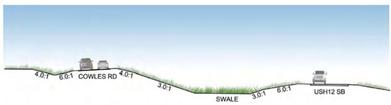
Typical Swale Section D 0 10' 20' 40'
