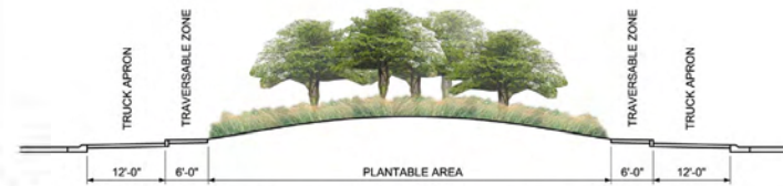
CTH W - Concept B Elevation
