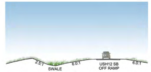
Typical Swale Section B 0 10' 20' 40'
