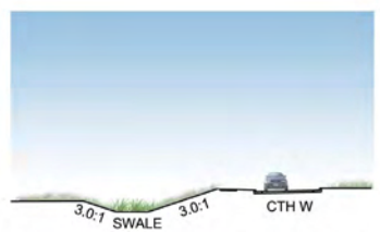
Typical Swale Section C 0 10' 20' 40'
