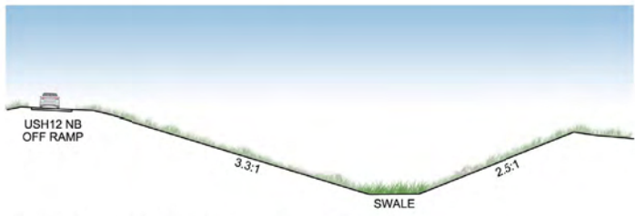
Typical Swale Section A 0 10' 20' 40'
