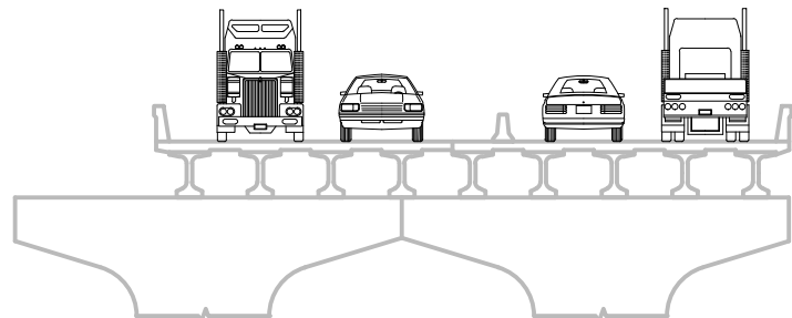
PROPOSED NEW NORTHBOUND BRIDGE
