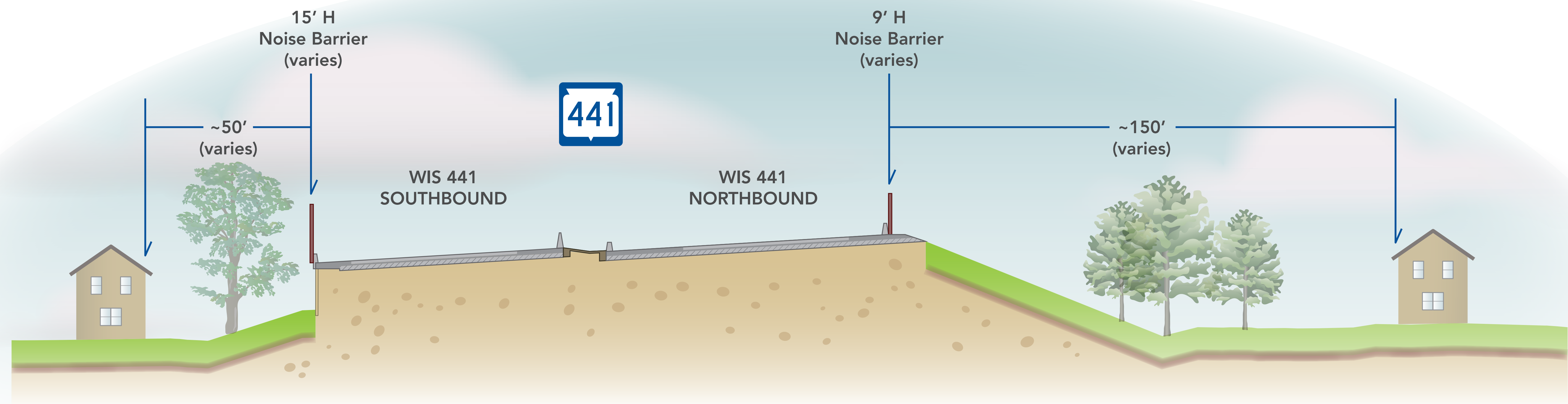
▲ Typical section (facing east)
