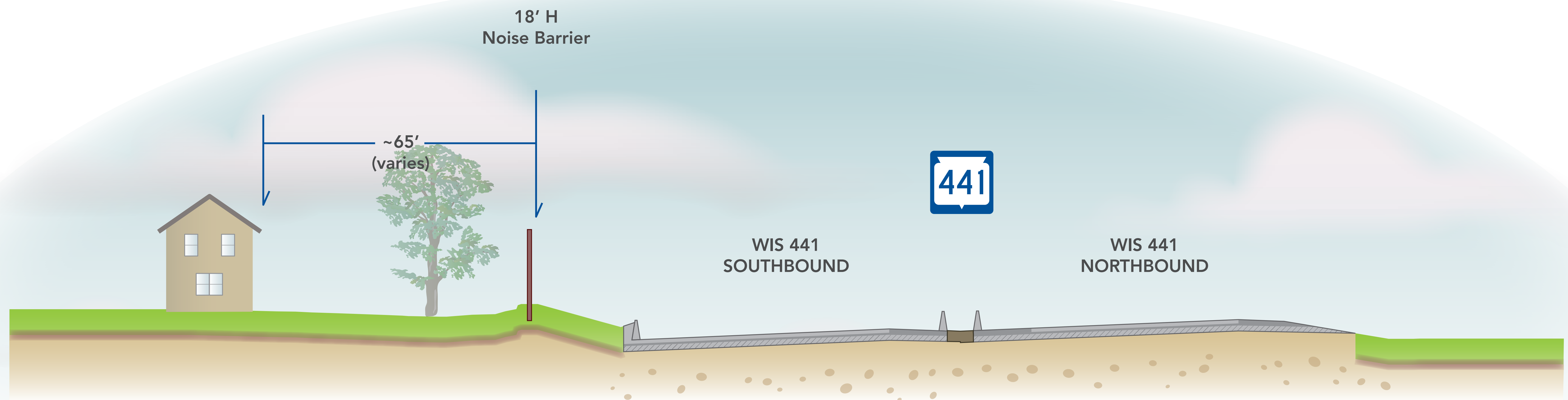
▲ Typical section (facing northeast)
