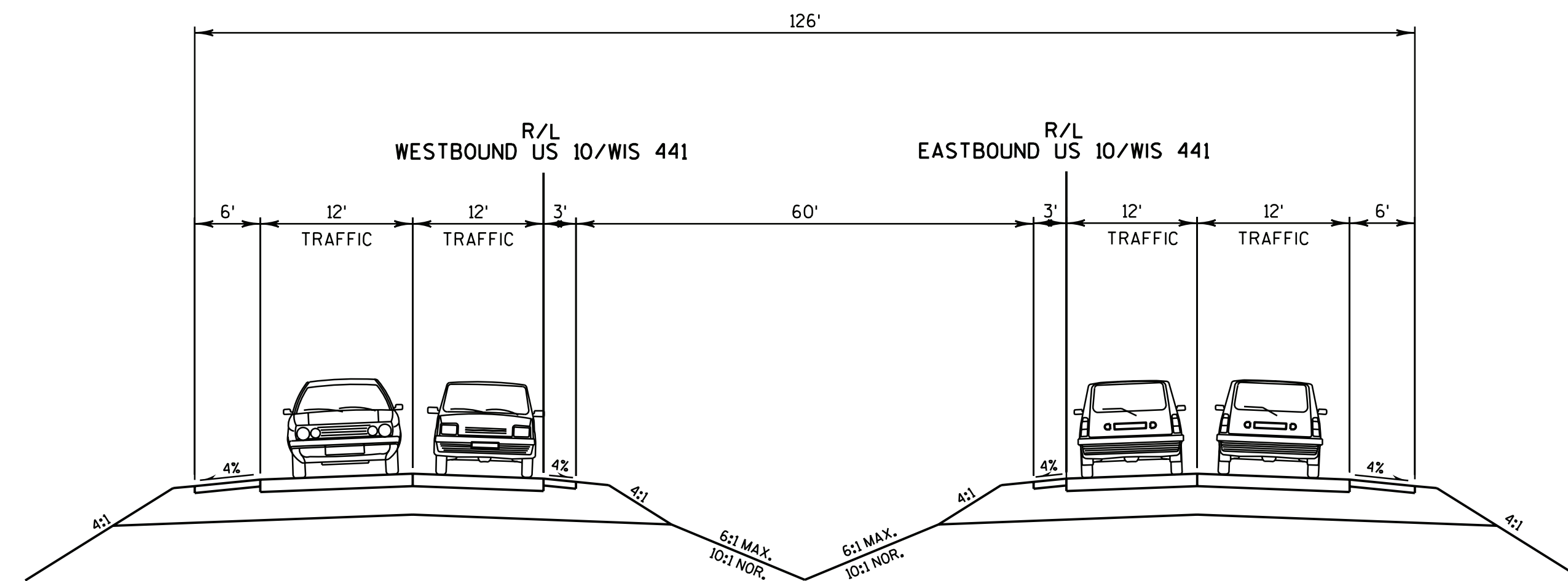
US 10/WIS 441 MAINLINE - EXISTING TYPICAL SECTION EASTBOUND AND WESTBOUND LANES
