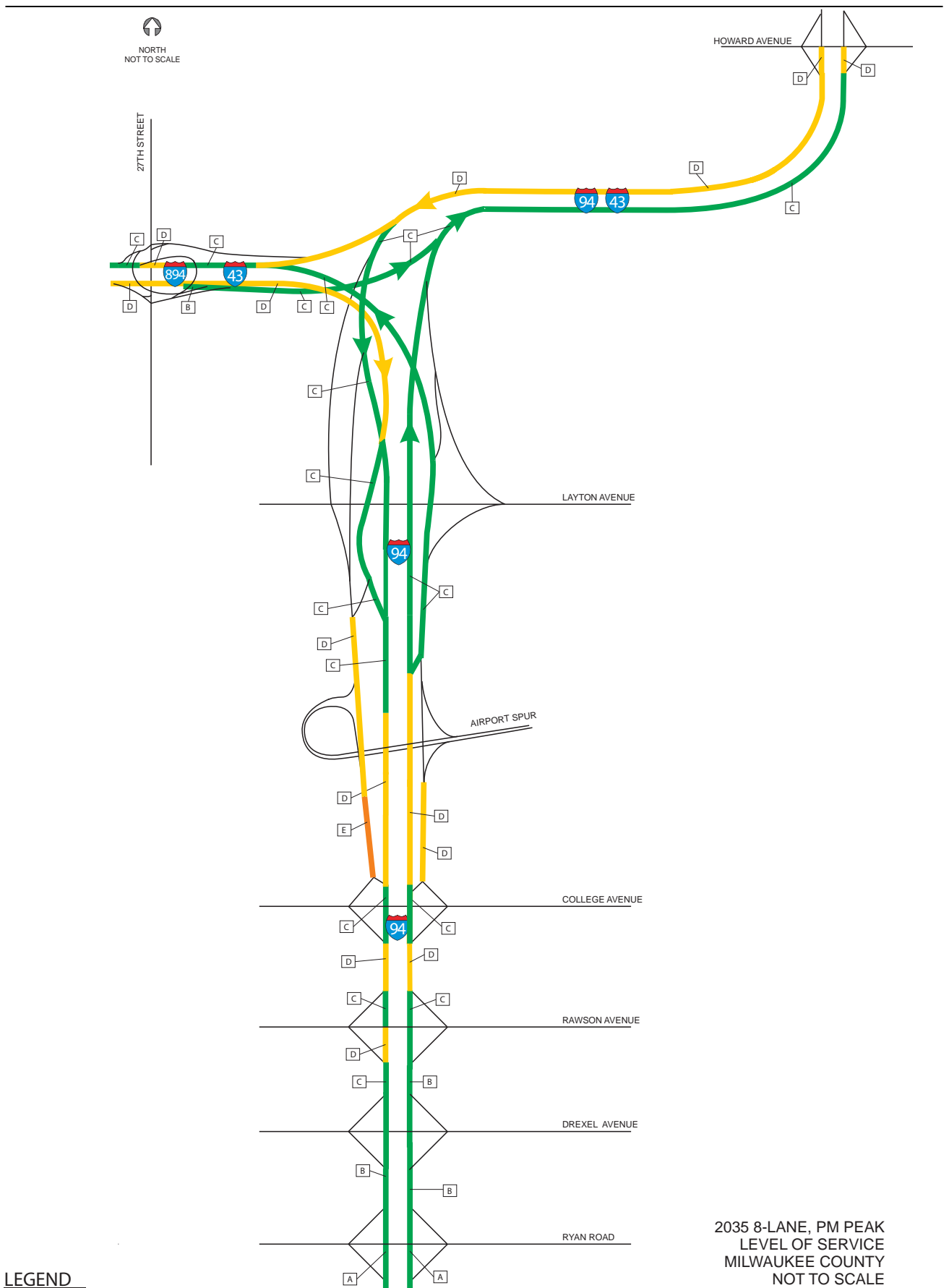
EXHIBIT 4-5 Safety and Design Improvements With Added Capacity Alternative
