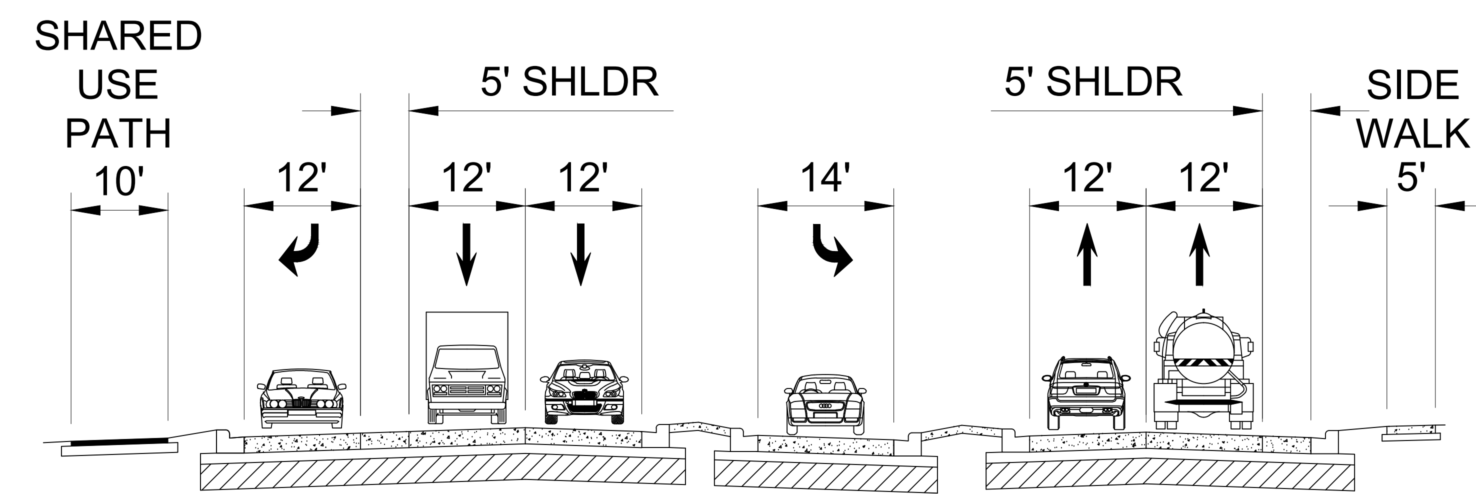
US 14 TYPICAL SECTION
