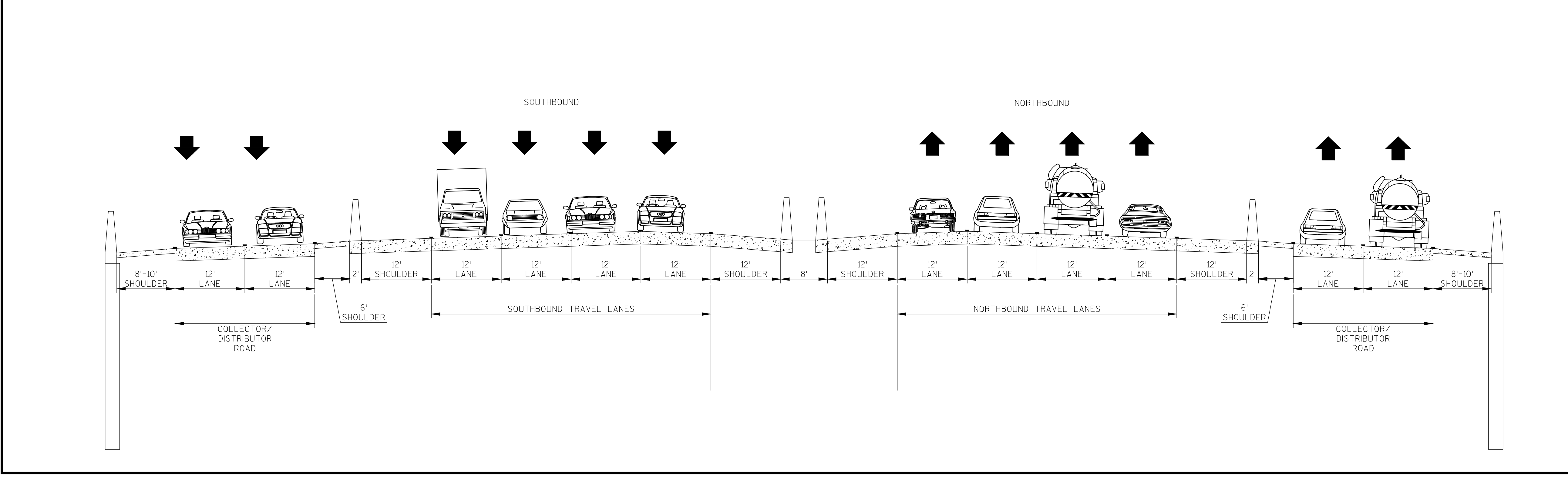
PROPOSED TYPICAL SECTION: I-39/90 (USH 14 - KENNEDY RD)
