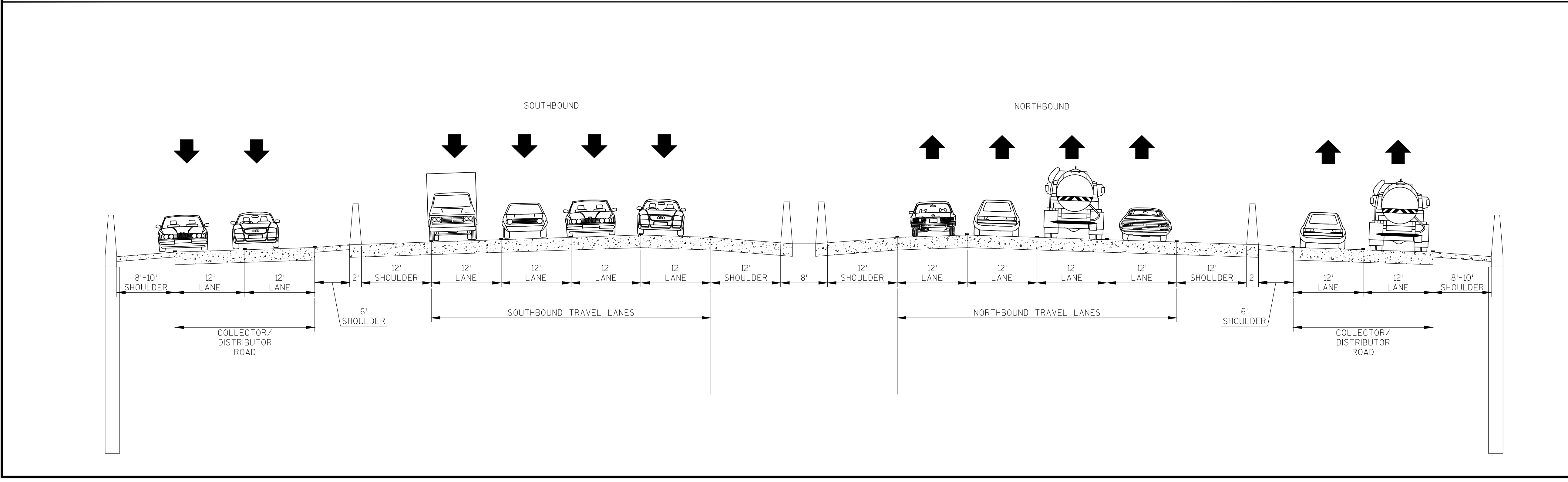
PROPOSED TYPICAL SECTION: I-39/90 (USH 14 - KENNEDY RD)
