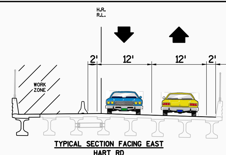
WORK ZONE TYPICAL SECTION: HART ROAD
