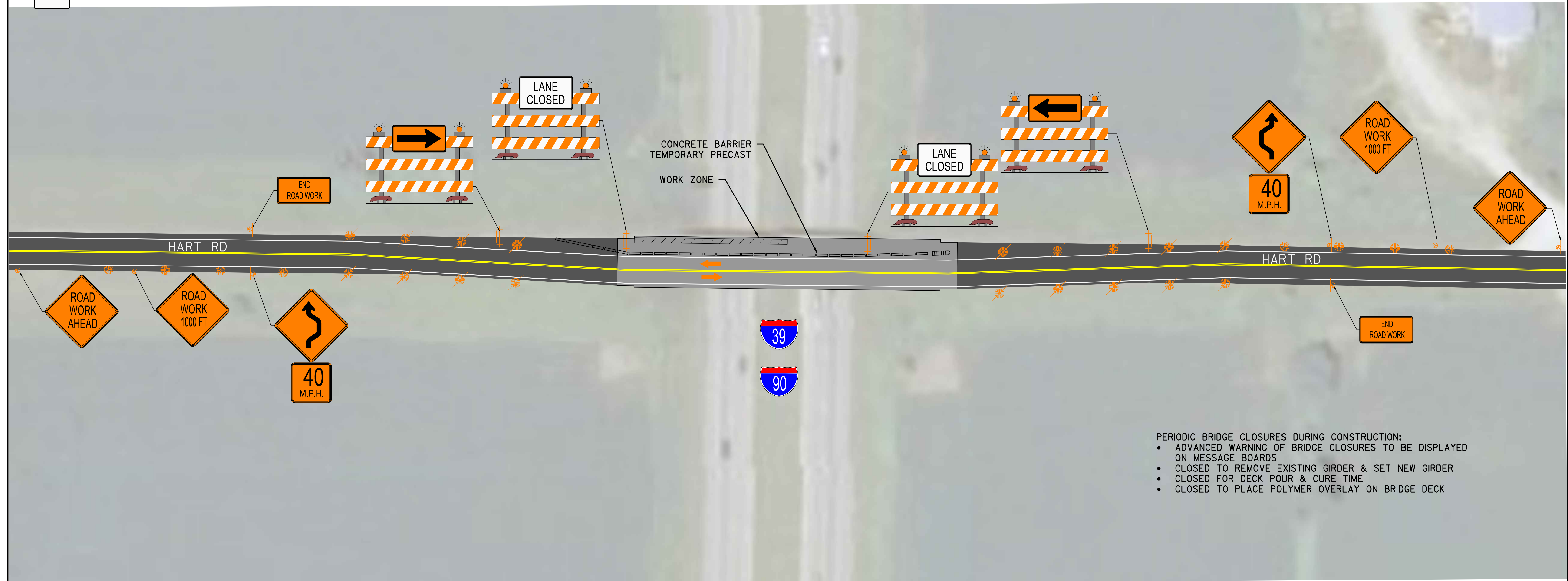
WORK ZONE TYPICAL SECTION: HART ROAD
